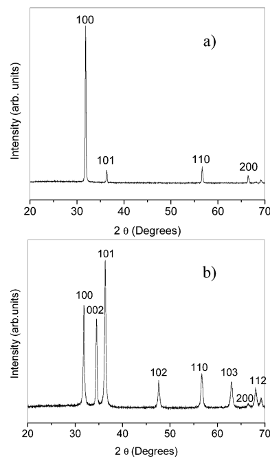
Fig. 1 XRD of (a) (100) oriented ZnO needles (b) ZnO sample (features corresponding to those of JCPDS card No. 36-1451).
